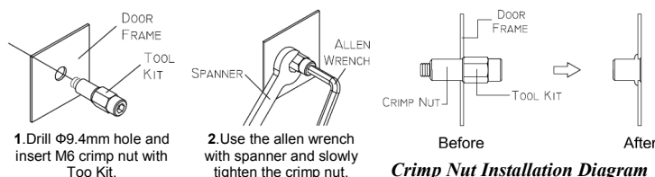
Crimp Nut Installation Diagram
